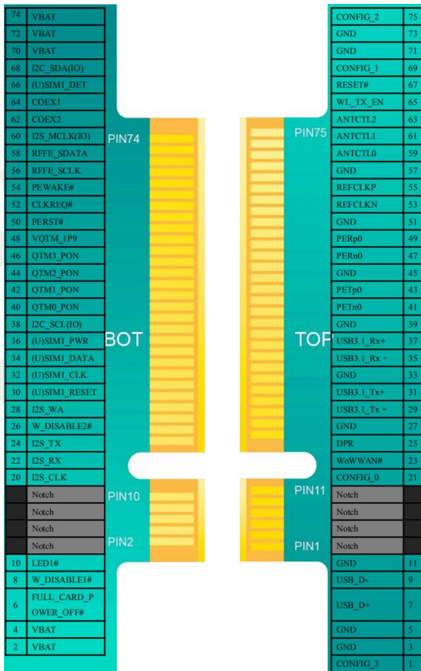
Figure 2: Pin assignment
