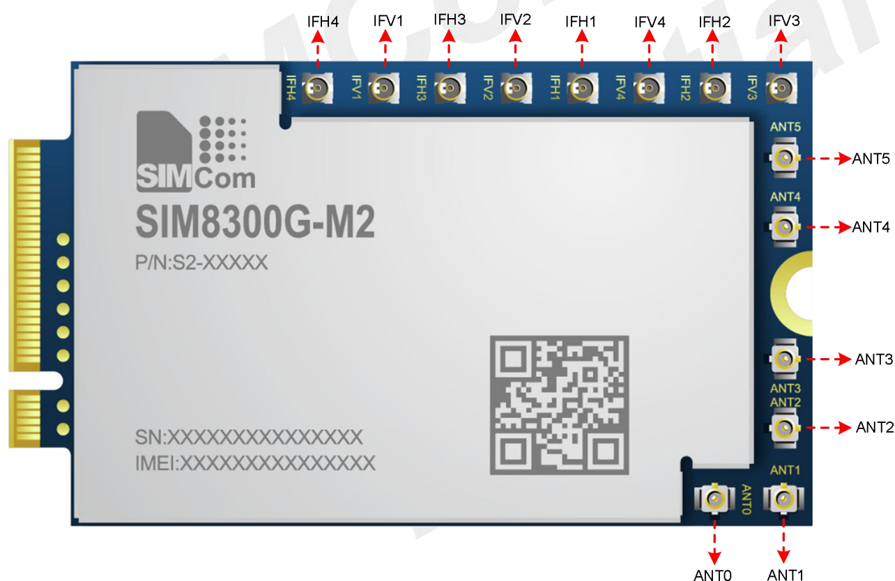
Figure 23: Antenna interfaces
