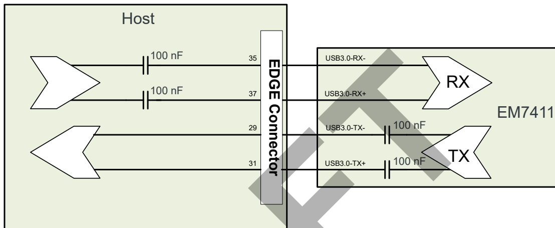
Figure 2-1: Recommended Capacitor Placement for USB3.0 Signals
