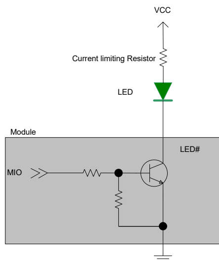
Figure 2-6: Example LED
