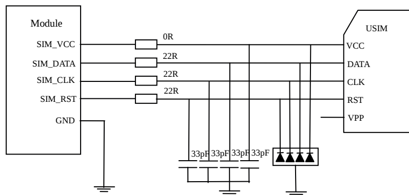
Figure 3- 14 USIM design circuit
