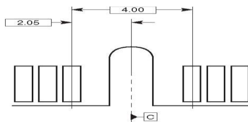
Figure 3- 1 TOP and BOTTOM of Pins
