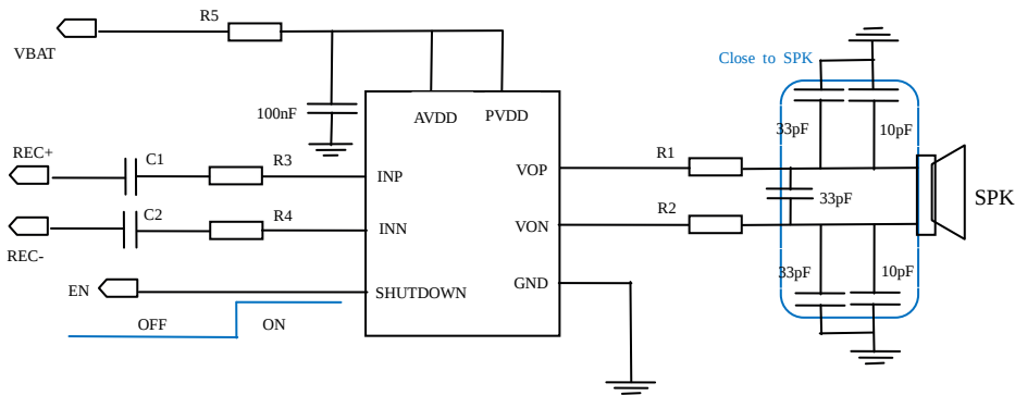
Figure 3- 19 External audio codec reference circuit
