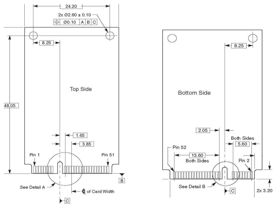
Figure 3- 1 TOP and BOTTOM of Pins
