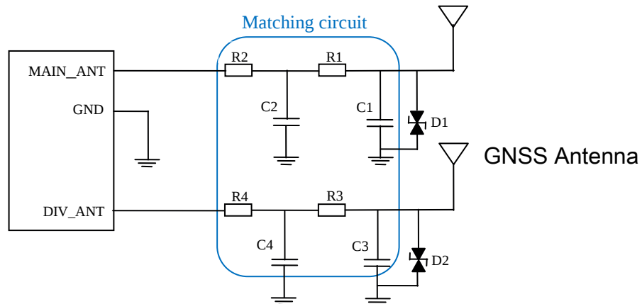
Figure 3- 24 Antenna matching circuit
