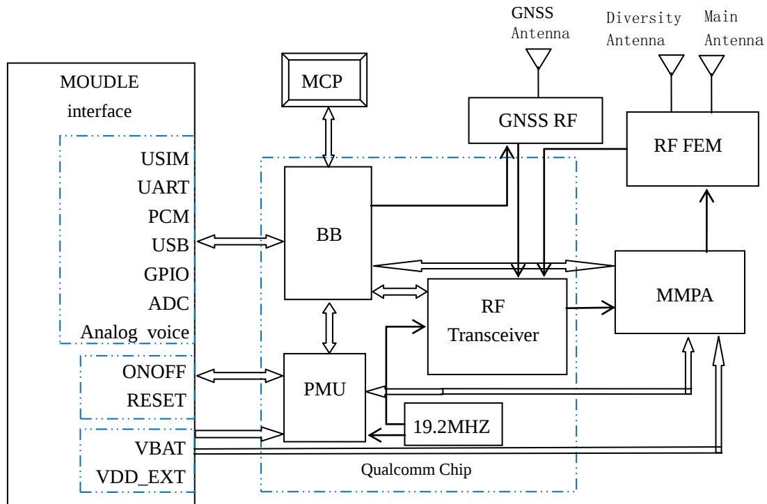
Figure 2- 1 CLM920_TE5 Functional Diagram
