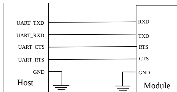
Figure 3- 12 UART serial port design
