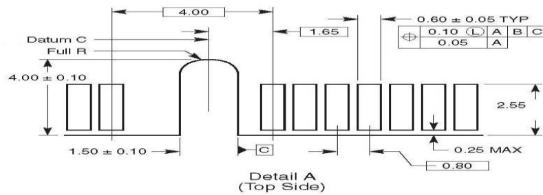
Figure 3- 2 TOP and BOTTOM in Detail A&B
