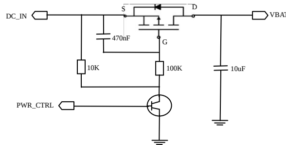
Figure 3- 7 Reference Design of MOS to control the power switch
