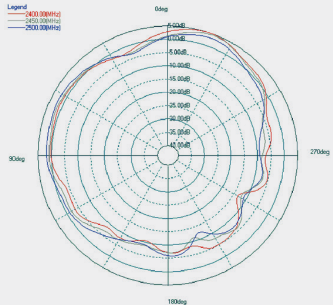
2.4G (PHI=90)
