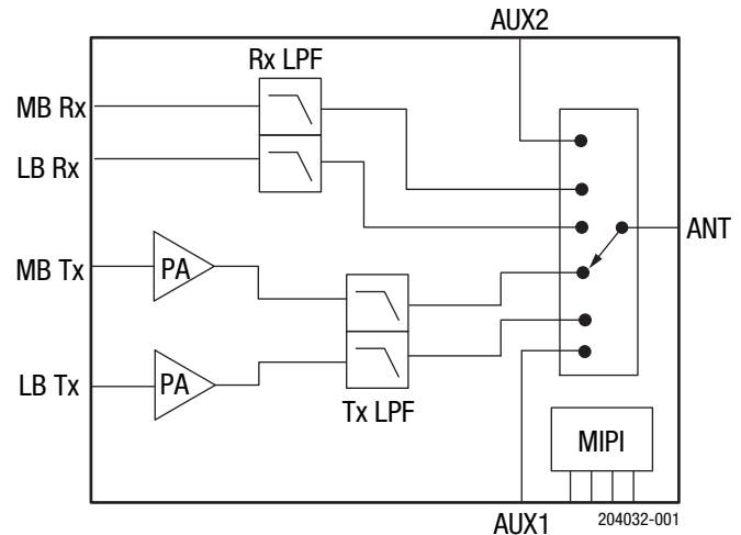
SKY68001-21 Functional Block Diagram
