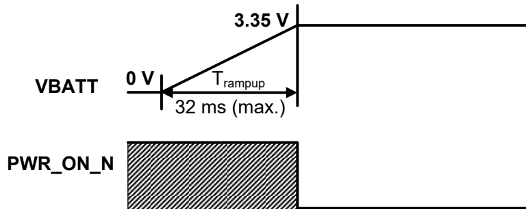
Figure 17. PWR_ON_N Sequence with T_{\text{rampup}}
