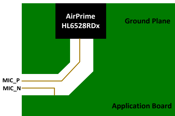
Figure 32. Single-Ended Audio Connection
