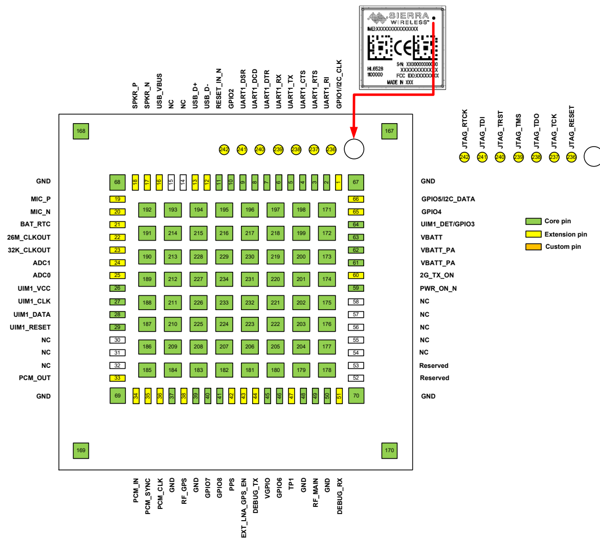
Figure 3. Pad Configuration
