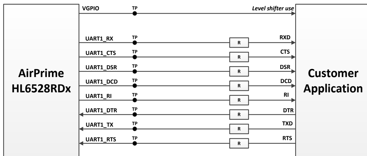
Figure 5. 8-wire UART Application Example
