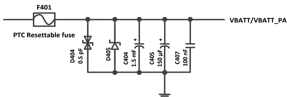
Figure 23. Voltage Limiter Example
