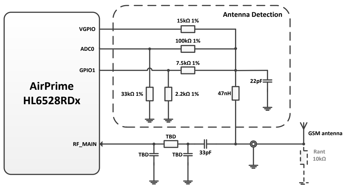
Figure 33. GSM Antenna Connection with Antenna Detection
