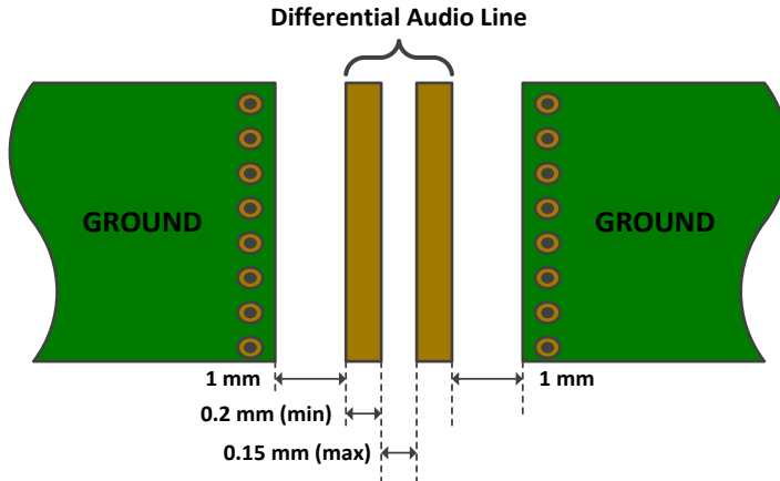
Figure 30. Audio Track Design
