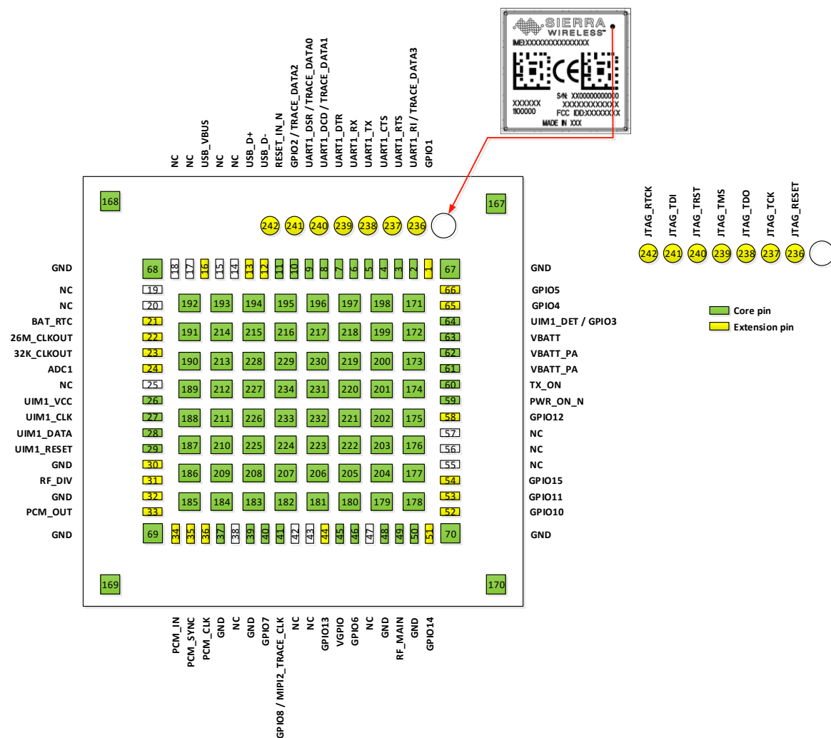
Figure 3. Pad Configuration
