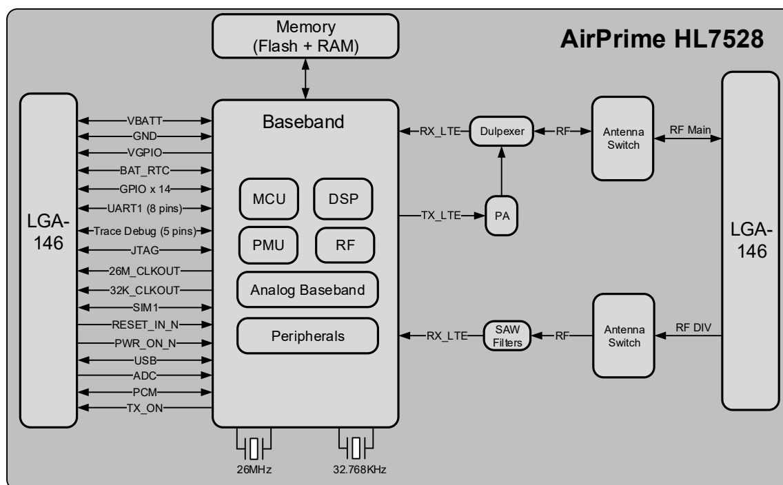
Figure 1. AirPrime HL7528 Architecture Overview
