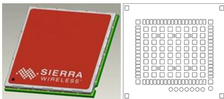
Figure 2. AirPrime HL7528 Mechanical Overview
