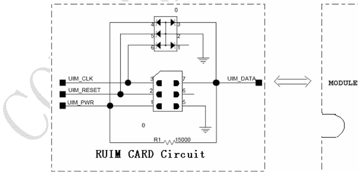
Figure 3-1 RUIM interface schematic on user's PC
